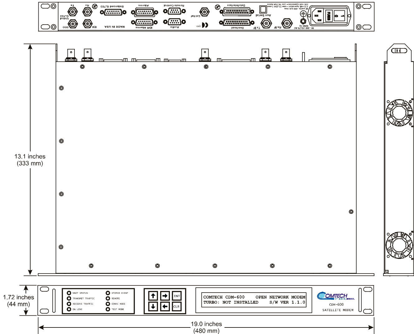
Figure 4-3. Dimensional Envelope
