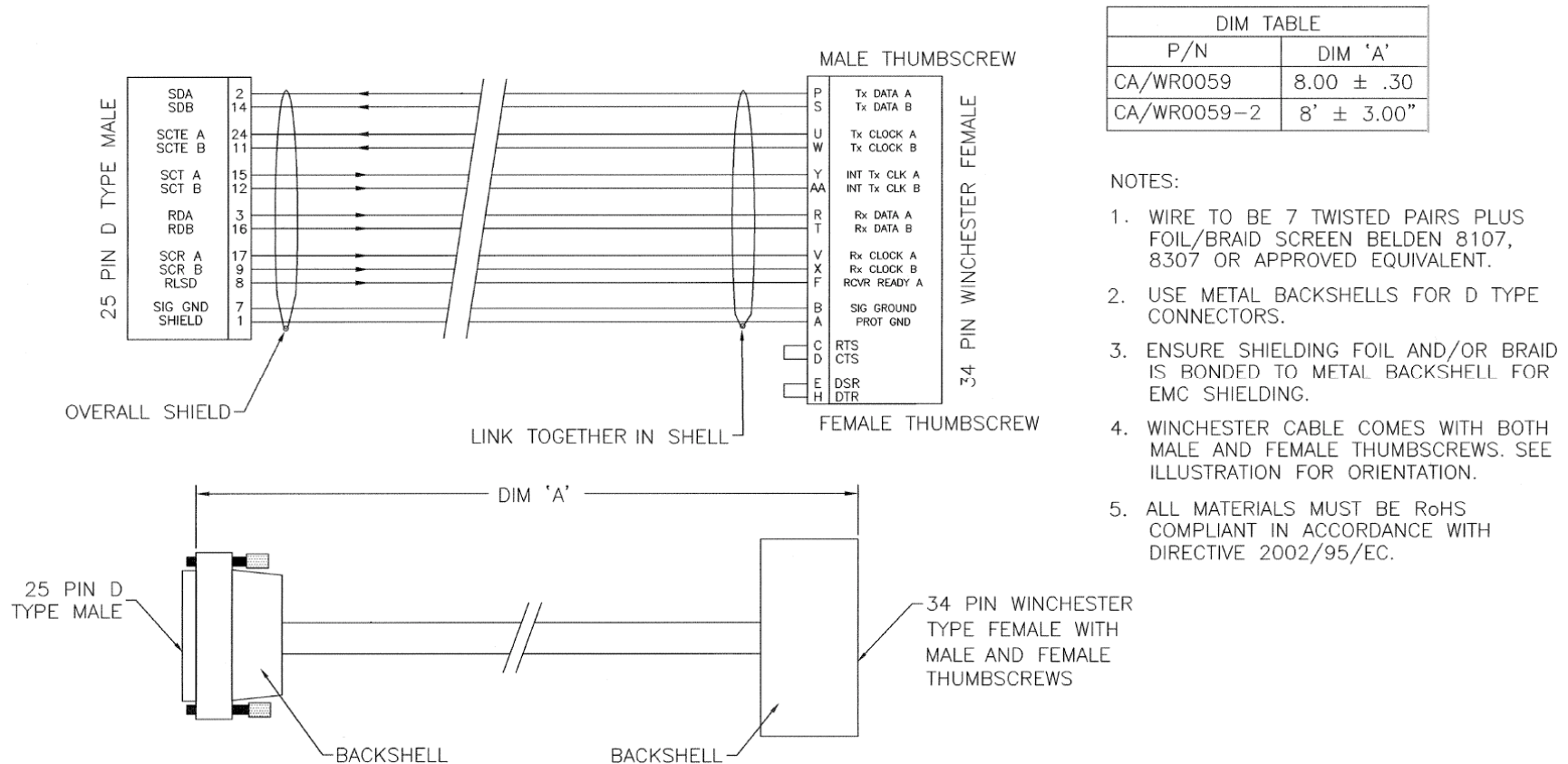
Figure A-2. DCE Conversion Cable: EIA-530 to V.35 (CA/WR0059)
