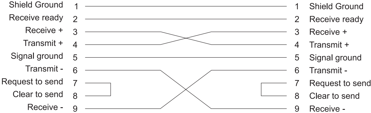
Figure 6. Master Slave interface cable diagram
